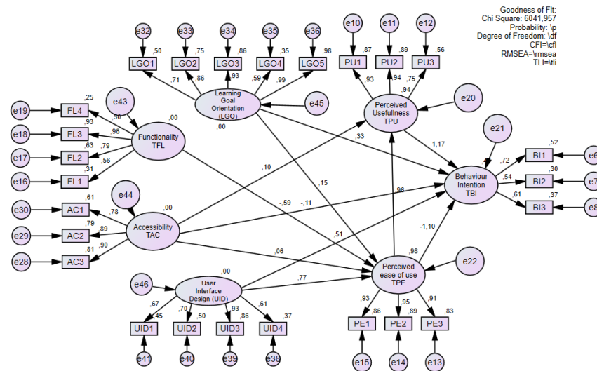
Fig. 4: Revision model
