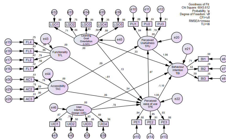
Fig. 5: Model Fit
