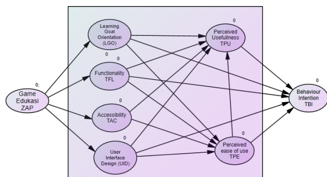
Fig. 2: Framework Research
