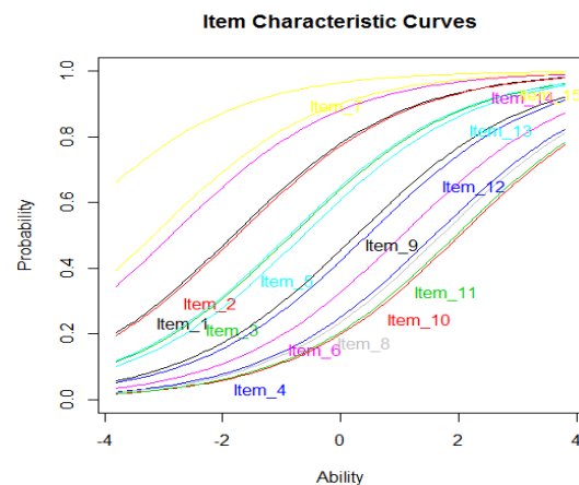
Fig. 2: Characteristic Curves for All Items
