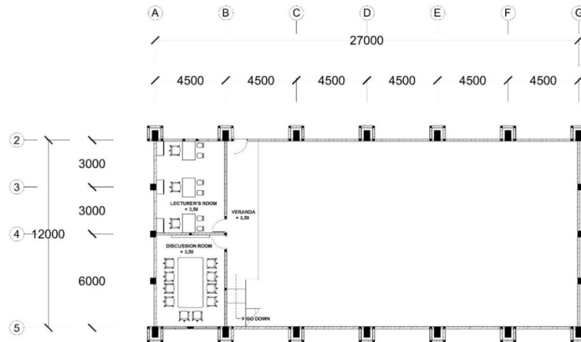
Fig. 3: Layout of the 2 nd Floor Building Materials Laboratory
